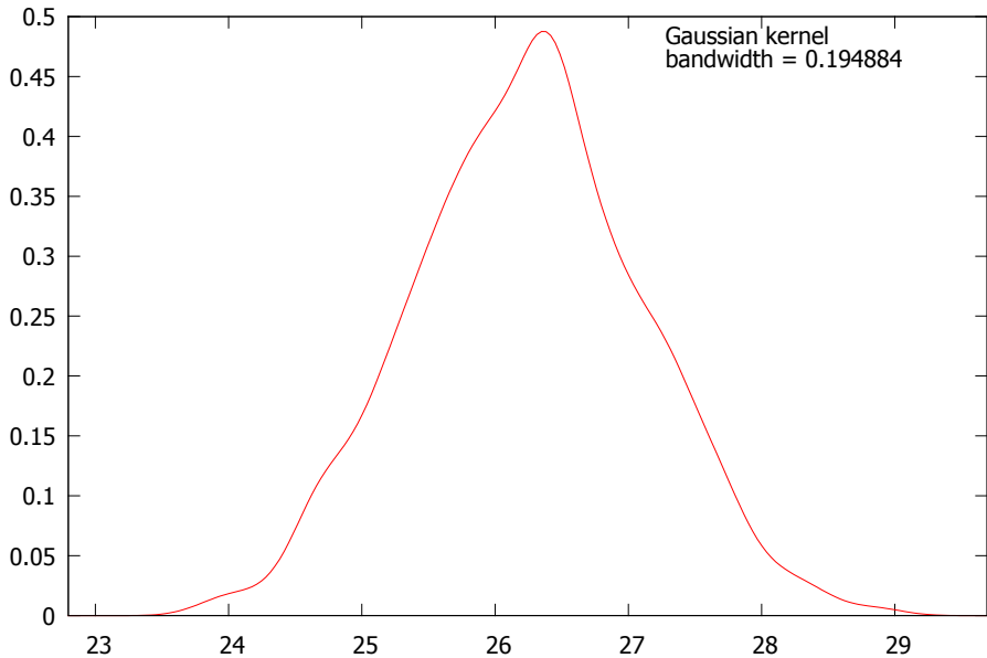
Estimated density of bootstrap t-ratio
