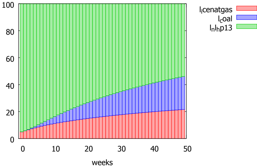
forecast variance decomposition for I_{nlhp13}
